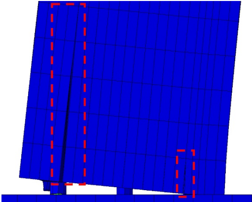
(b) Crack patterns based on FE model
